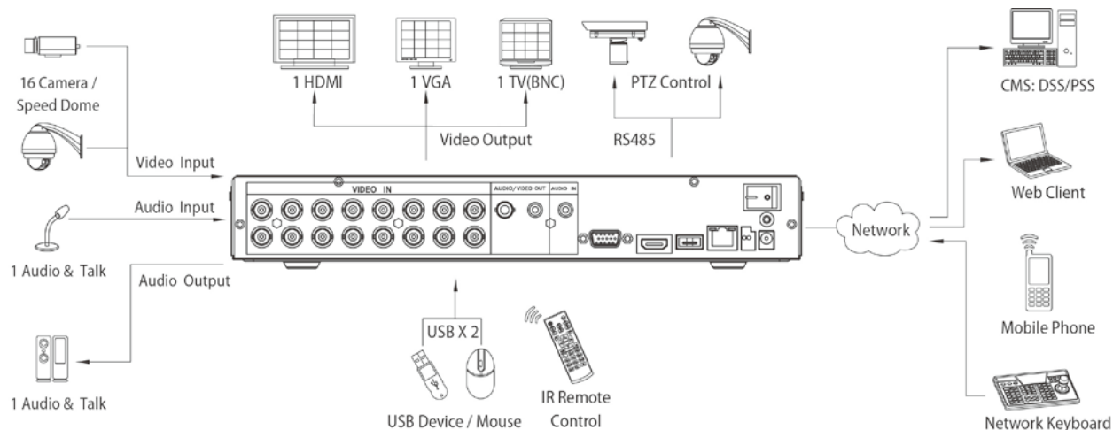
DVR5116H System Connection
